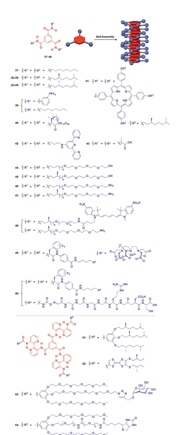
Fig. 9 Schematic structures of BTA-( 37–49 ) and extended BTA-based ( 50–54 ) helical 1D supramolecular scaffolds (red), and examples of functional molecular units (blue) assembled with the scaffolds.
