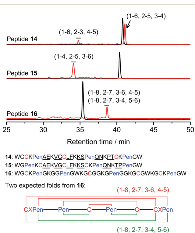
Fig. 5 Amino acid sequences of peptides 14–16 (from N- to C-terminus); randomized amino acid residues were underlined (AE VG LFK KS QN PT/TP). In peptide 15, the residues threonine (T) and proline (P) following the lysine residue were exchanged to facilitate the analysis of disulfide pairings by the tryptic digestion HPLC and mass spectrometry. The length of the each variable segment in 16 was shortened by depletion of one amino acid residue to facilitate the synthesis. Chromatograms showing the oxidation of 14–16 (10 \mu M) in 0.2 mM GSSG (100 mM phosphate buffer, pH 7.4) (black line: before oxidation; red line: 2 h after oxidative folding). For the folding of 15 and 16, other fully oxidizing isomers were not detected, and impurity peaks in the chromatograms should mainly come from trapped folding intermediates, which restrict overall yields of the expected folds. Disulfide pairings were established by tryptic digestion HPLC and mass spectrometry (Fig. S44–S50†).
