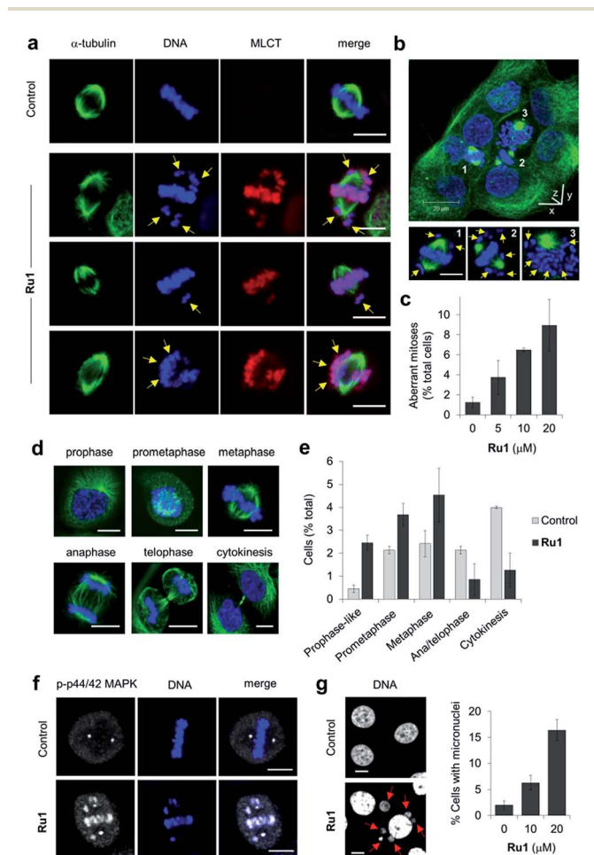
Fig. 4 (a) Misaligned metaphase chromosomes (yellow arrows) in OE21 cells treated with Ru1 (20 μM, 4 h). After fixation, cells were stained for α-tubulin (green) and DNA (DAPI, blue). MLCT (metal to ligand charge-transfer) emission of Ru1 included. (b) 3D representation of Ru1 -treated OE21 cells (20 μM, 24 h) prepared from z-stack images. Non-aligned chromosomes in labelled cells shown by yellow arrows. (c) Quantification of aberrant mitoses in Ru1 -treated OE21 cells (24 h). Data average of two independent experiments ± S.D., >200 cells were counted for each condition. (d) CLSM images of mitotic stages of OE21 cells. (e) Quantification of mitotic sub-populations in Ru1 -treated OE21 cells (20 μM, 24 h). Data are expressed as a percentage of total cell population. Data average of two independent experiments ± S.D., >200 cells counted per experiment. (f) Localisation of phospho(p)-p44/p42 MAP kinase in metaphase OE21 cells treated with Ru1 (20 μM, 24 h), as determined by immunofluorescence (AlexaFluor594, white). DNA staining (DAPI, blue) included for reference. (g) Formation of micronuclei (red arrows) in OE21 cells treated with Ru1 (20 μM, 24 h). Data average of two independent experiments ± S.D. where >100 cells were counted for each condition. Scale bars = 10 μm.
