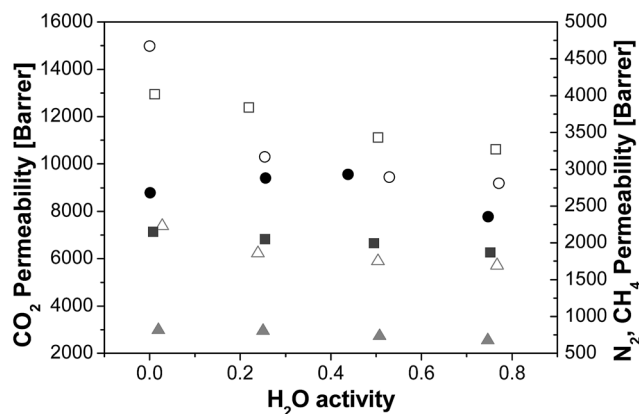
Fig. 1 Permeability (barrer) at different relative humidity ( T = 35\text{ }^{\circ}\text{C} , p = 1 bar) for the zeolite A/PTMSP MMM (full symbols) and PTMSP membranes (void symbols). N 2 (grey triangles), CH 4 (dark grey squares) and CO 2 (black circles).
