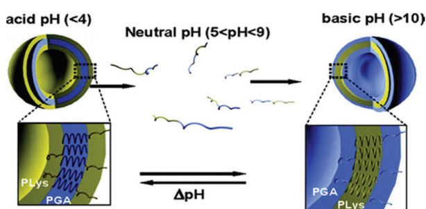
Fig. 3 Schematic representation of pH-regulated schizophrenic vesicles from the self-assembly of the diblock copolyptide \text{PGA}_{15} - \text{b} - \text{PLys}_{15} in water. Reprinted with permission from ref. 15. Copyright (2005) American Chemical Society.
