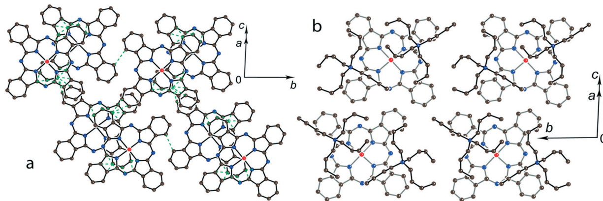
Fig. 3 (a) View of the phthalocyanine layer composed of the \pi -stacking [(\text{Ti}^{\text{IV}}\text{O}(\text{Pc}^{3-}))_2]_2 dimers in 2 . 12 Short van der Waals C...C,N contacts are shown by green dashed lines. (b) Projection of the \text{Bu}_4\text{N}^+ layer on the phthalocyanine layer. Only one phthalocyanine from the dimer is shown (bonds are shown in grey).
