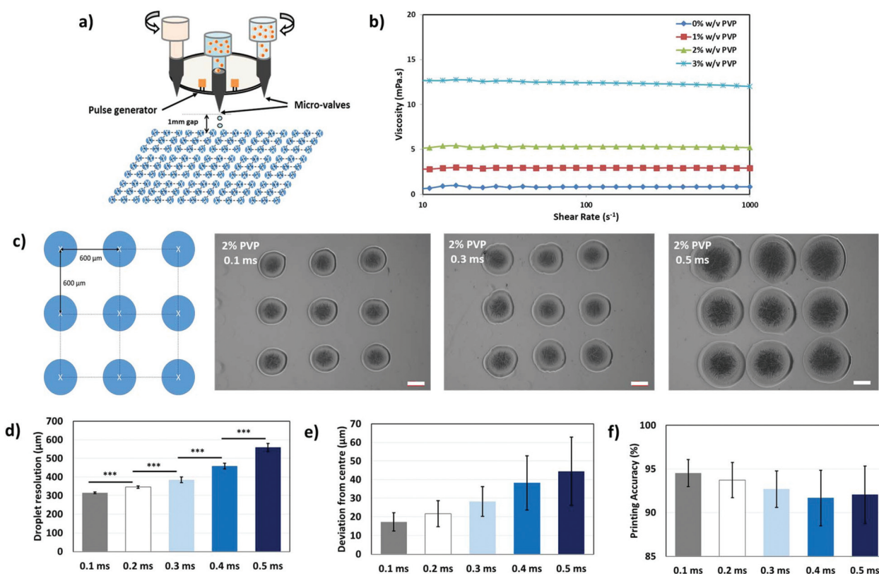
Fig. 3 (a) Schematic drawing of drop-on-demand microvalve-based printing for PVP-based bio-inks. (b) Rheological characterization of different PVP-based bio-inks (0–3% w/v) from 10–1000 s -1 . (c) Arrays of 3 × 3 PVP droplets are printed at a constant spacing of 600 μm (centre marked by white X) and representative images of the printed PVP droplets at different valve opening times (VOTs) from 0.1–0.5 ms; scale bar: 200 μm. ImageJ analysis of the (d) droplet resolution, (e) deviation from the centre and (f) printing accuracy.
