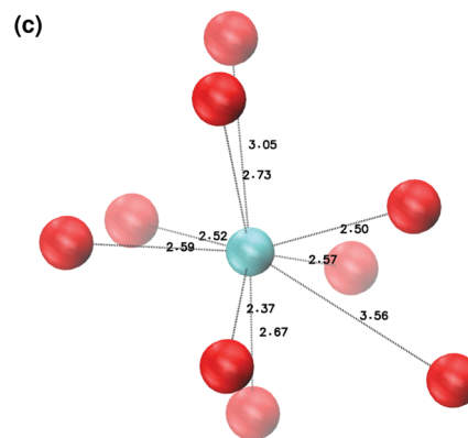
Fig. 10 Solution III: (a) aggregates after 5 ns; (b) detail of one of the Posner-like clusters formed with formula \text{Ca}_9(\text{PO}_4)_6 ; (c) distances between the central Ca1 and the neighbouring oxygens. Colour key Ca: light blue, P: green, O: red, atoms not forming Posner's clusters: grey.
