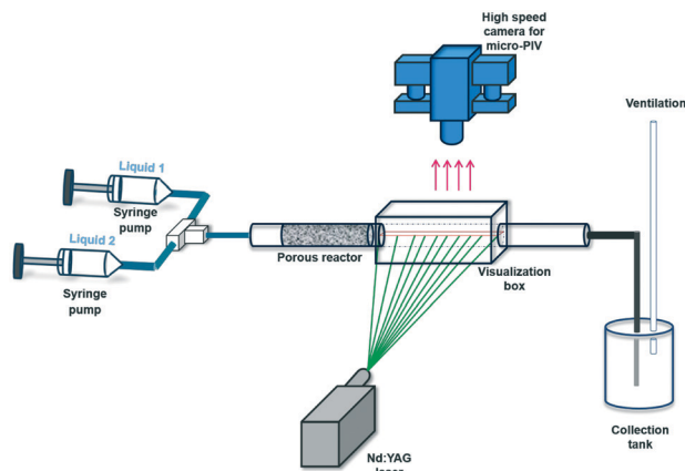
Fig. 3 Schematic representation of the experimental setup for optical measurements.
