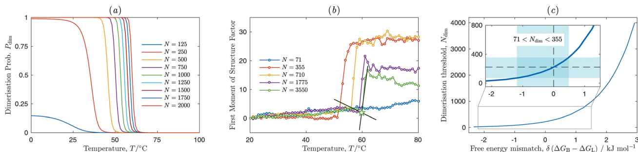
Fig. 5 Temperature-dependent dimerisation of vesicles. (a) Simulated dimerisation probability as a function of temperature and number of linkers (per type) N . Model parameters: N_v = 8004 , L = 3\sigma . (b) Experimental first moment of the structure factor in aggregating LUVs as a function of temperature and N . Data are recorded while heating up aggregated samples. Straight lines (solid) are used to fit the curves just below and just above the melting transition, and identify the melting temperature (star symbol). Samples with N = 71 never show aggregation, while samples with N = 355 always aggregate. Samples with N = 177 aggregate in 2 out of 5 independent repetitions of the experiment (not shown for clarity), indicating that N = 177 is close to the threshold value for vesicle dimerisation N_{\text{dim}} . First moment curves collected on cooling/heating ramps are smoother due to the slow aggregation kinetics, and are unsuitable to accurately locate the phase transition. If multiple cooling/heating ramps are performed, we observe a systematic shift of the melting temperature towards lower T . We ascribe this effect to vesicle degradation resulting from the repeated exposure to high temperatures. (c) Predicted N_{\text{dim}} as a function of an hypothetical unbalance \delta(\Delta G_B - \Delta G_L) between bridge and loop-formation free energies, where \delta(\Delta G_B - \Delta G_L) = 0 marks our original choice. In the inset the shaded region highlights the experimentally determined range for the threshold value 71 < N_{\text{dim}} < 355 .
