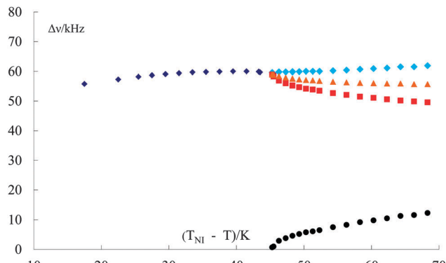
Fig. 12 The quadrupolar splittings, \Delta\nu , for CB6OCB- d_2 shown as a function of the shifted temperature (T_{NI} - T) in the nematic and twist-bend nematic phase. In the N_{TB} phase the two splittings from the prochiral deuterons ( \blacklozenge , \Delta\nu_+ , and \blacksquare , \Delta\nu_- ) are also shown as the mean splitting (\Delta\nu_+ + \Delta\nu_-)/2 ( \blacktriangle ) and as the chiral splitting (\Delta\nu_+ - \Delta\nu_-) ( \bullet ).
