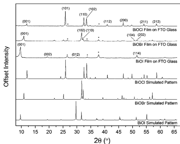
Fig. 3 PXRD of BiOX ( X = \text{Cl, Br, I} ) films deposited on FTO glass from the AACVD reaction of \text{BiX}_3/\text{DMF} in air at 300^\circ\text{C} along with simulated BiOX patterns. The asterisked peaks correspond to positions of reflections from the F : SnO (FTO) substrate.
