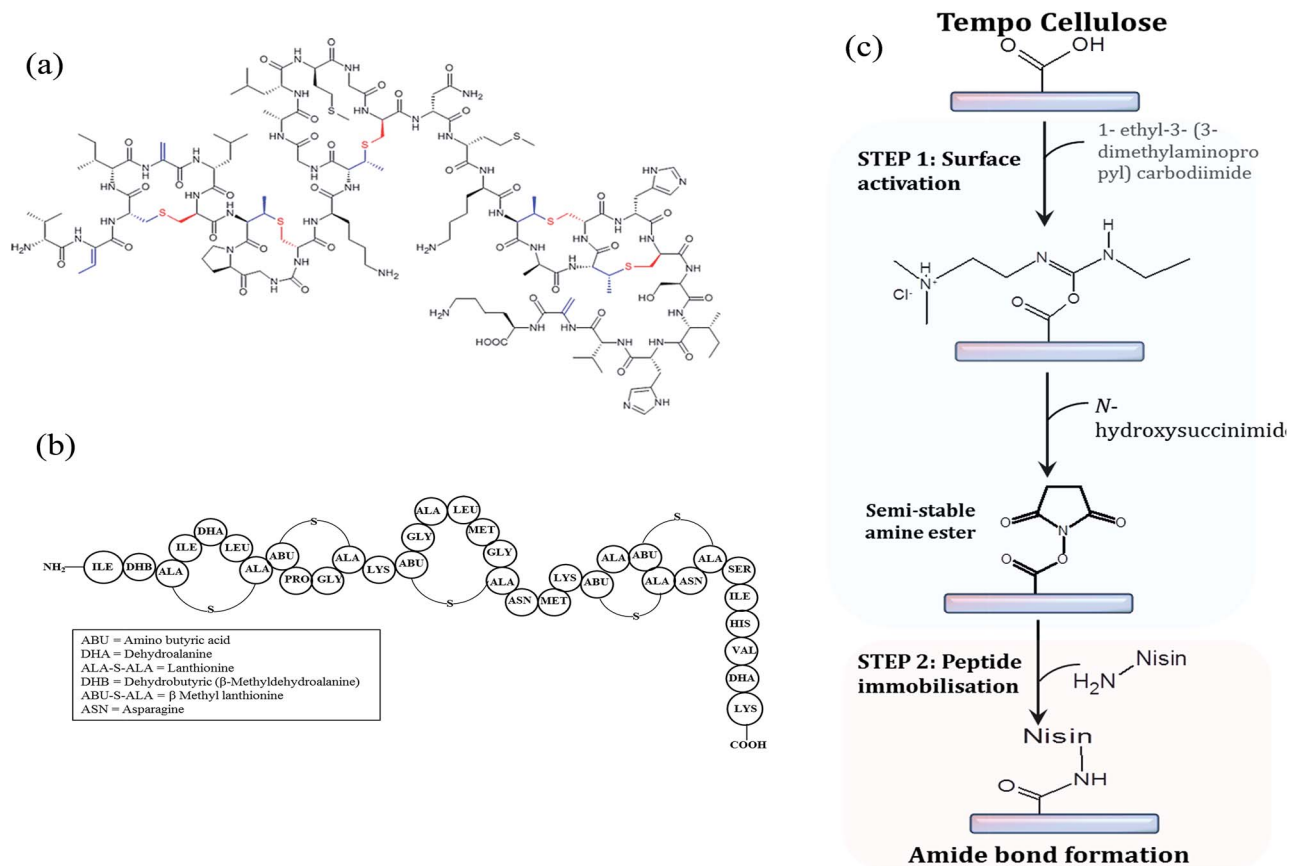
Fig. 3 (a) Chemical structure of the lantibiotic nisin Z (b) primary structure of nisin Z (nisin Z contains asparagine instead of histidine at position 27) (c) schematic illustration of the main steps involved in the grafting of peptide nisin Z on the surface of tempo cellulose.
