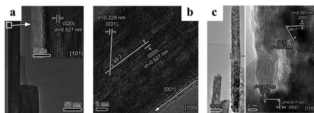
Fig. 3 (a) Low-magnification TEM image of a single \beta -FeOOH nanorod viewed along the [101] direction. The insert HRTEM image indicates that the nanorod exposes the {010} planes. (b) Another HRTEM image viewed along the [100] orientation, also showing the preferential exposure of the {010} planes, (c) low- and high-magnification TEM images of a single \gamma -Fe 2 O 3 nanorod, indicating the dominant exposure of the {110} and {001} planes (modified with permission from ref. 39, copyright 2012 Wiley-VCH).
