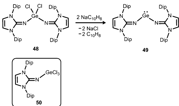
Scheme 11 Reductive dehalogenation of the dichlorogermane 48 to the bisiminogermerylene 49 . The trichlorogermane 50 .
