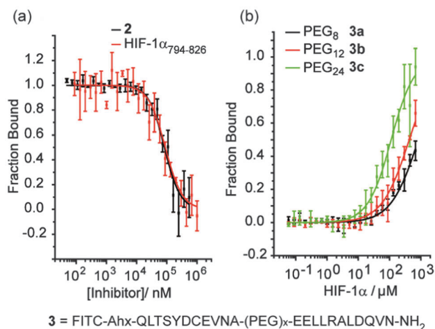
Fig. 2 Biophysical screening of HIF-1α peptides and hybrids, HIF-1α 794–826 , 2 and 3a–c (a) fluorescence anisotropy (FA) competition data for inhibition of p300/FITC-HIF-1α C-TAD for HIF-1α 794–826 and 2 (b) (FA) binding data for 3a–c to p300 (schematic structure shown below).
