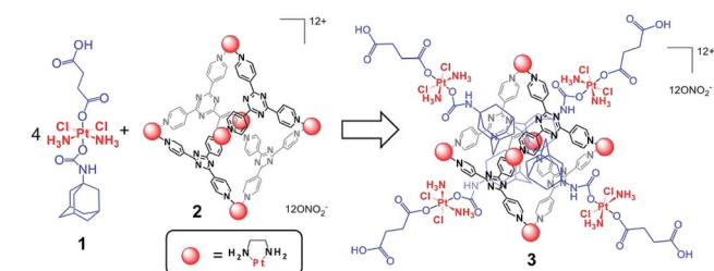
Scheme 1 Representation of the host-guest complex ( 3 ) assembled from the Pt(IV) prodrug ( 1 ) and the Pt(II) cage ( 2 ).
