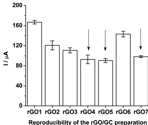
Fig. 11 ASWV peak currents of Pu(IV)/Pu(III) redox couple recorded on seven rGO/GCs in the final test solution ( i.e. ; sample + 3.047 mg\ g^{-1} of standard Pu). The error bars represent the standard deviation for ten repetitive measurements. The arrows show the rGO/GCs selected for the ANOVA test.
