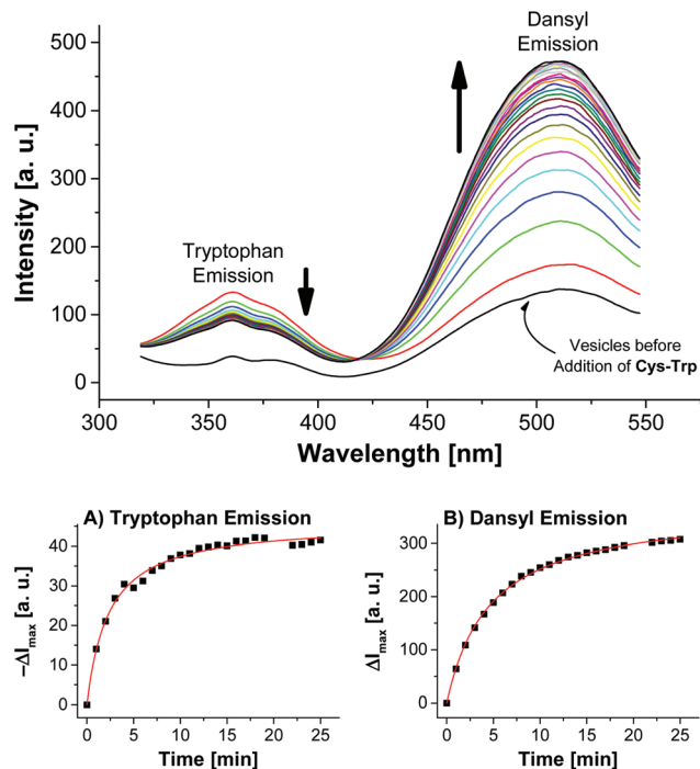
Fig. 5 Top: Time-dependent fluorescence spectra of vesicles V-Dans after addition of 3.0 mol% of peptide Cys-Trp ( \lambda_{\text{exc}} = 280 nm). Bottom: course of surface reaction as evidenced by the emission signals of either the tryptophan or dansyl dye.
