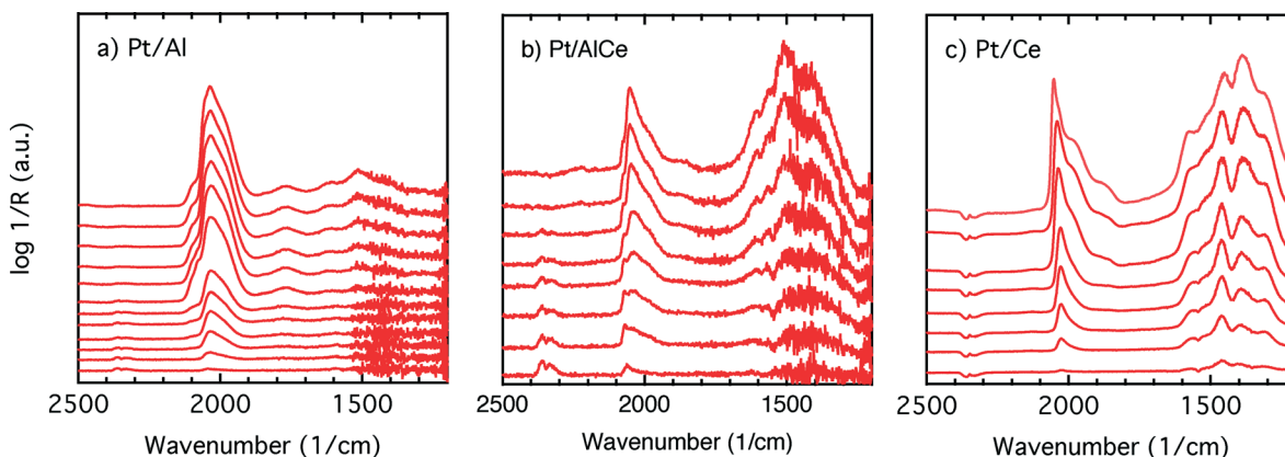
Fig. 6 Evolution of IR bands in the wavenumber region 1200\text{--}2500\text{ cm}^{-1} for (a) Pt/Al, (b) Pt/AlCe and (c) Pt/Ce catalysts exposed to 0.05% CO after initial pretreatment in 0.1% methane and 0.3% oxygen for 30 min at an inlet gas temperature of 400\text{ }^{\circ}\text{C} .
