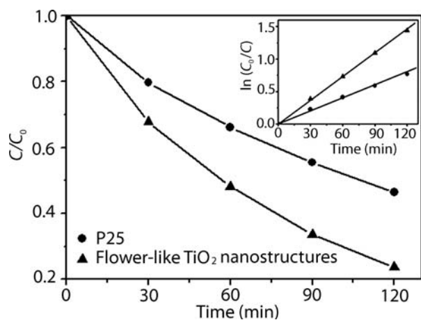
Fig. 3 The variation of MB concentration by photoelectrocatalytic reaction with P25 TiO 2 powders and flower-like TiO 2 nanostructures. The inset shows the pseudo-first-order kinetic rate plots for the photochemical degradation of MB.
