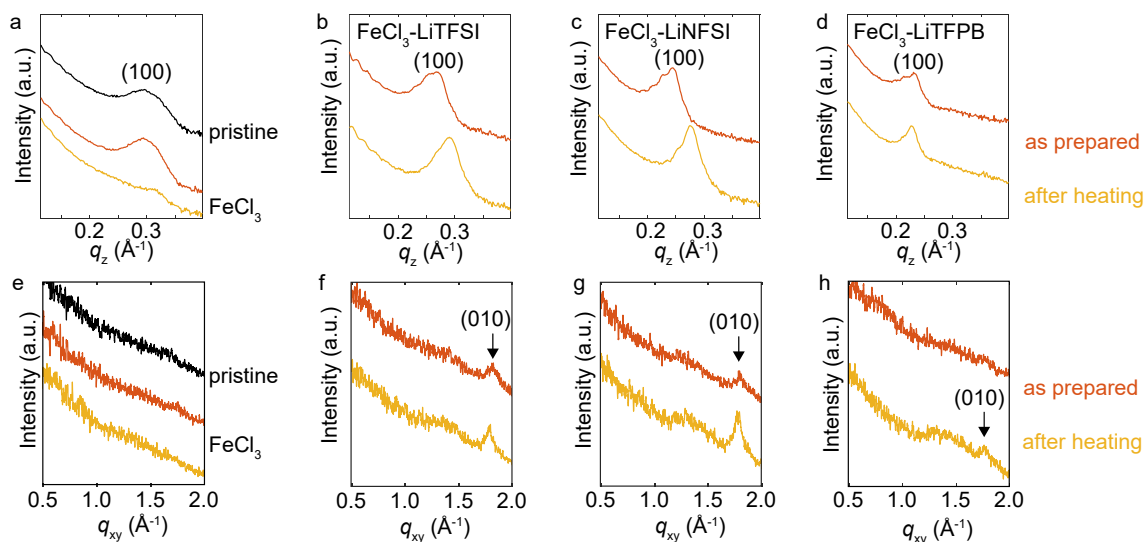
Fig. 4 XRD measurements of the doped PQT thin films. Intensities for the (a-d) out-of-plane and (e-h) in-plane directions. Orange plots were obtained from thin films after treatments with FeCl 3 or combinations of FeCl 3 and additional salts. Yellow plots were obtained after heating the treated samples at 125 °C under air.
