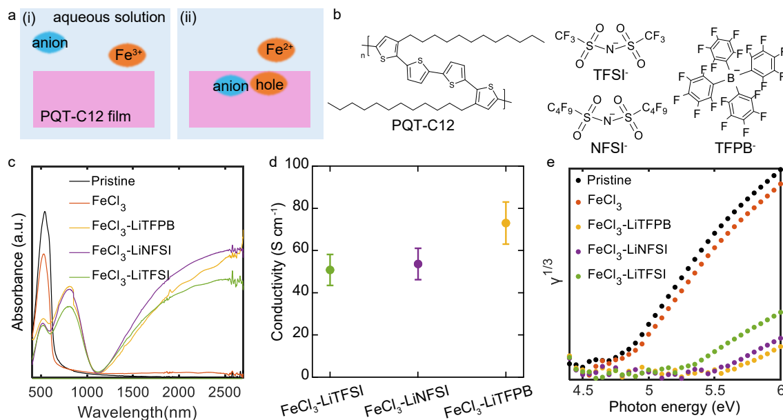
Fig. 1 Doping of PQT thin films. (a) A model of possible chemical doping mechanism with the illustrations of (i) initial and (ii) final state of doping system. (b) The molecular structures of employed materials. (c) UV-Vis spectra of the treated and untreated PQT thin films. The gap at 800 nm is due to the change of detector. (d) Conductivity of PQT thin films after the chemical doping process. \text{FeCl}_3 and the denoted salts were dissolved in doping solutions. The two-terminal geometry with channel length of 400 \mu\text{m} and width of 2 \text{ mm} was employed. Three samples were measured for each condition, where the error bar shows one standard deviation. (e) PYS spectra of the treated and untreated PQT thin films.
