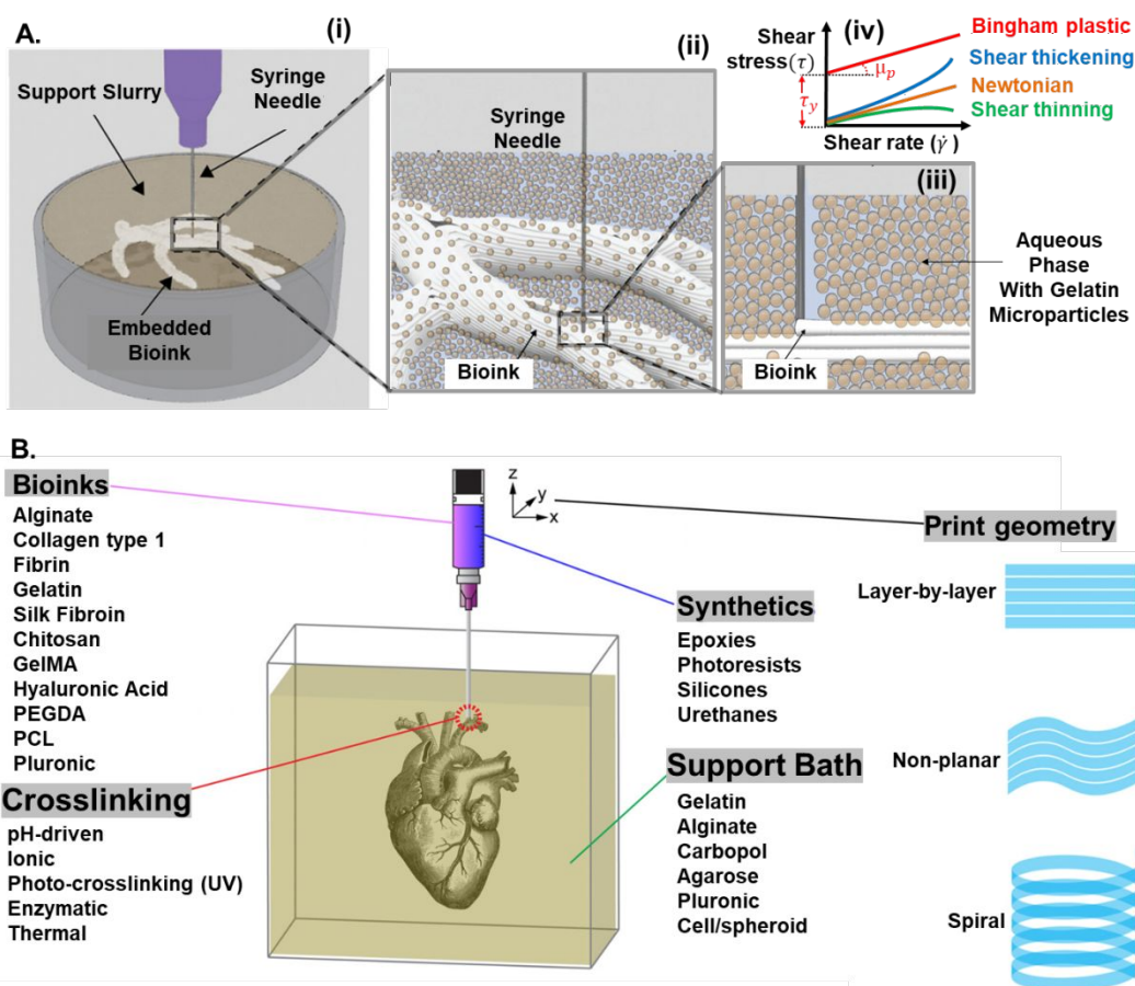
Figure 1. Embedded extrusion 3D bioprinting: (A) A print container is filled with a yield-stress gel microparticle support matrix to serve as the embedding medium for the intended components (i), the aqueous phase of the support matrix can be tuned to drive crosslinking/gelation of the nozzle-extruded bioink as the microparticles support the print during layer-by-layer deposition (ii), as the needle moves through the support matrix, the microparticles yield providing a space for the extruded bioink and subsequently heal behind the needle providing support to the curing bioink (iii); the flow behavior of the support bath is Bingham plastic (iv); (B) Classification of different synthetic or natural bioinks, different crosslinking routes, different paths for printing, and matrix compositions (adapted from Ref. [9] with permission from AIP Publishing, copyright 2021).
