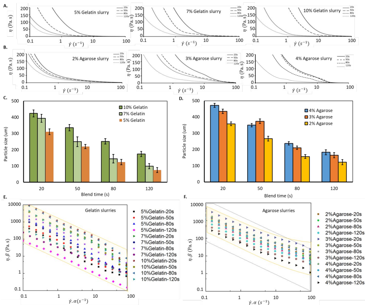
Figure 2. FRESH-specific rheological response of different slurries made of (A) 5, 7, and 10 % w/v gelatin and (B) 2, 3, and 4 % w/v agarose, utilizing 20, 50, 80, and 120 s blend time; the average microparticle size obtained after blending the (C) gelatin and (D) agarose slurries; the calculated master curve locus obtained for (E) gelatin and (F) agarose slurries.
