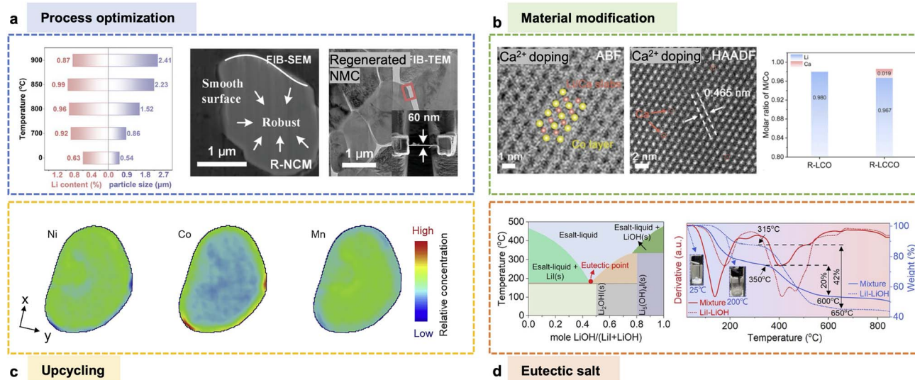
Fig. 6 Progress on molten salt regeneration. (a) Process optimization. Temperature effects on Li content and particle size. Reprinted with permission from ref. 188. Copyright 2024 Wiley. (b) Material modification. Annular bright-field (ABF)-STEM, HAADF-STEM, ICP result of \text{Ca}^{2+} doped LCO. Reprinted with permission from ref. 185. Copyright 2024 Elsevier. (c) Upcycling. Ni, Mn and Co relative concentrations distribution over a particle slice revealed by XRF. Reprinted with permission from ref. 190. Copyright 2022 Elsevier. (d) Eutectic salt. Phase diagram and TG-DTG curves of the \text{LiI-LiOH} eutectic salt system. Reprinted with permission from ref. 194. Copyright 2022 American Chemical Society.
