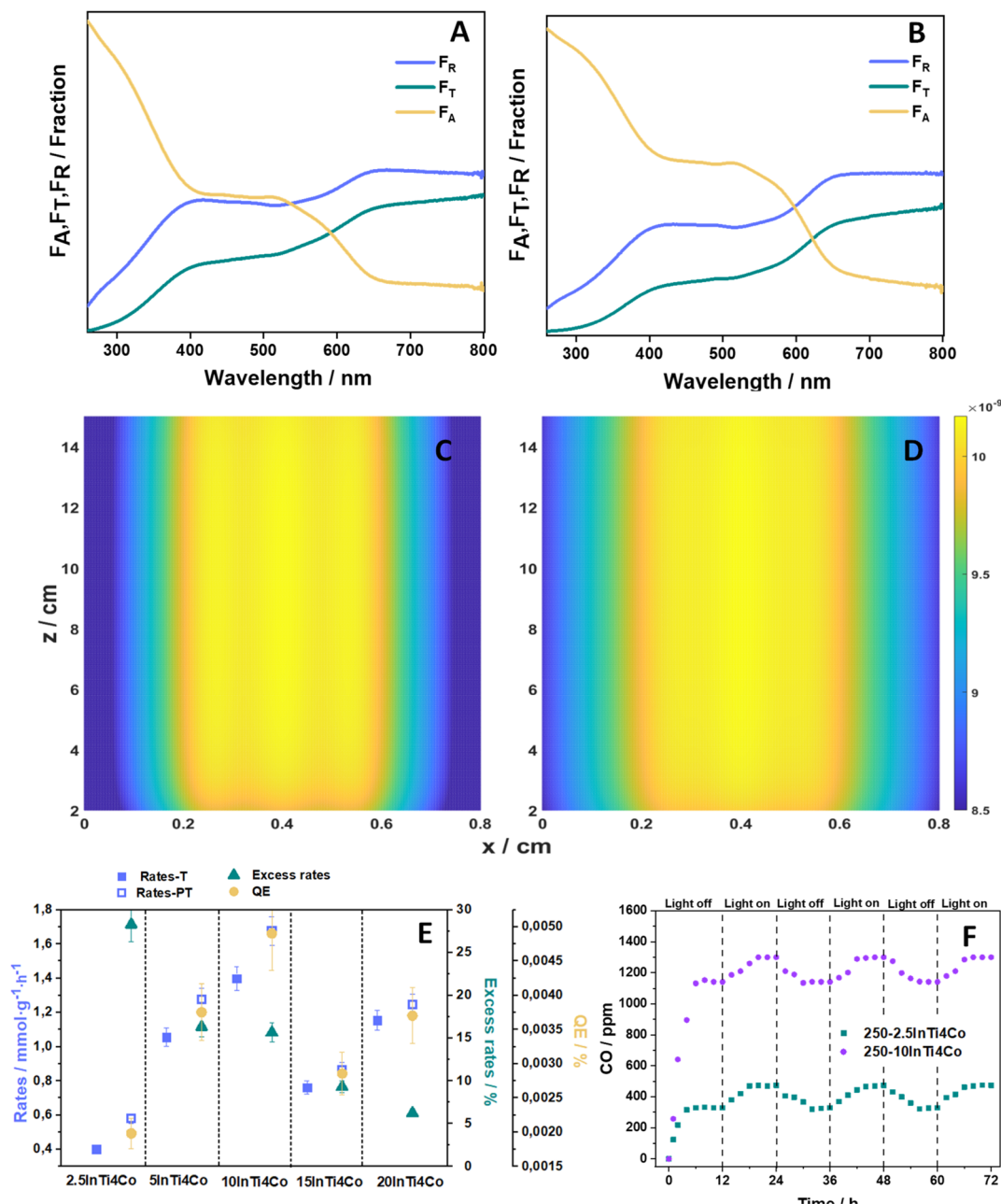
Fig. 5 (A and B) Fraction of light absorbed, transmitted or reflected by the 2.5In-Co-Ti and 10In-Co-Ti samples, respectively. (C and D) Local photon absorption rate at 250 °C (einstein m -2 s -1 ) under irradiation for the 2.5In-Co-Ti and 10In-Co-Ti samples, respectively. (E) Reaction rates, excess rates and quantum efficiency for xIn-Co-Ti samples. (F) Long-term operation tests for selected samples under light off/on cycling conditions.
