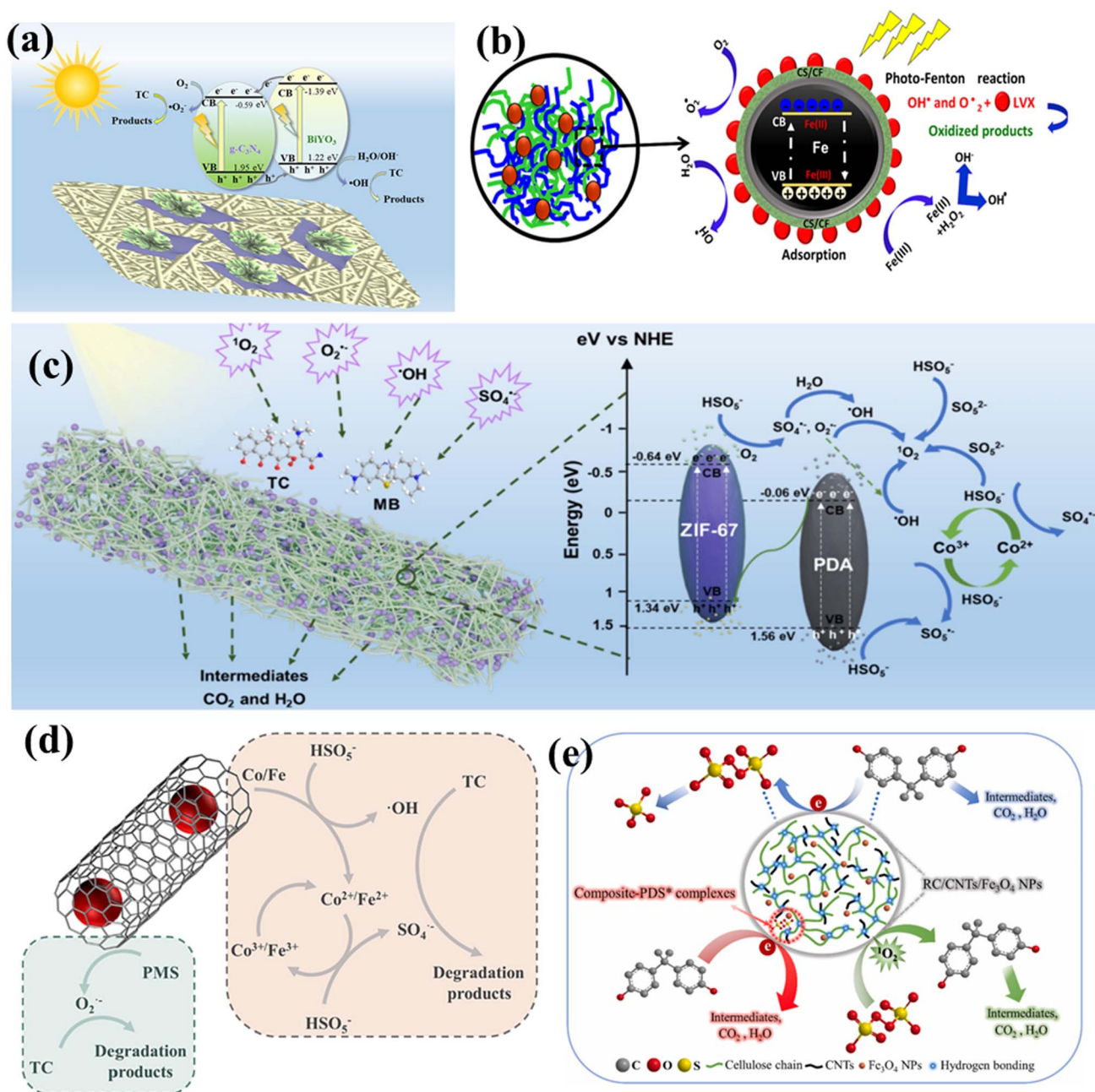
Fig. 12 (a) Diagram of tetracycline degradation using \text{GCN}/\text{BiVO}_4 via photocatalysis. Reprinted with permission from ref. 136, Elsevier (2023). (b) Photo-Fenton-assisted mechanism for the degradation of LVX using \text{Fe}^0/\text{chitosan}/\text{cellulose} green hybrid structures. Reprinted with permission from ref. 202, Elsevier (2024). (c) Mechanism for the degradation of tetracycline using the PMS system. Reprinted with permission from ref. 232, Elsevier (2025). (d) Schematic of proposed tetracycline degradation using the \text{CoFe}_{0.8}\text{@NCNT@CA}/\text{PMS} catalytic system. Reprinted with permission from ref. 233, Elsevier (2022). (e) Diagram of bisphenol-A degradation using \text{RC}/\text{CNT}/\text{Fe}_3\text{O}_4 nanoparticles. Reprinted with permission from ref. 234.
