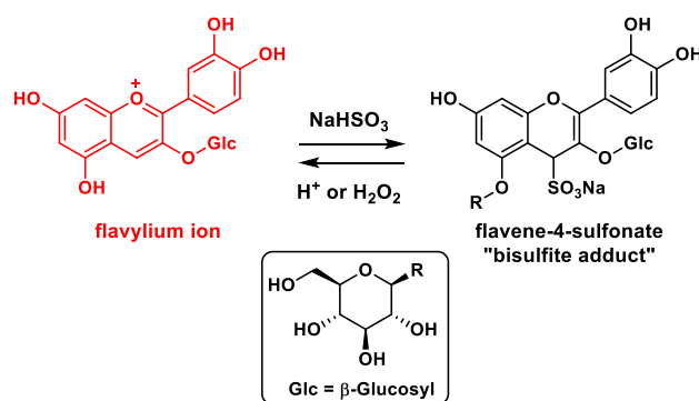
Fig.9 The reaction of the flavylium ion form of cyanidin-3-glucoside with sodium bisulfite to form the corresponding flavene-4-sulfonate or "bisulfite adduct". Typical conditions for the reverse reaction are also shown.
