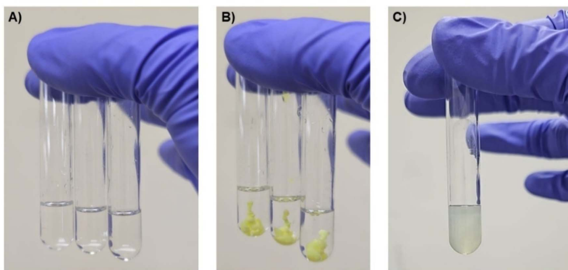
Fig. 5 Yellowish precipitate formed between DES and the Folin-Ciocalteu reagent. (A) DES based on ChCl: lactic acid with different water percentages, 0, 15, and 30 wt%. (B) F-C reagent precipitate in DES. (C) DES with F-C reagent after vortexing, the turbidity is so high that it renders measurement by spectrophotometry impossible.
