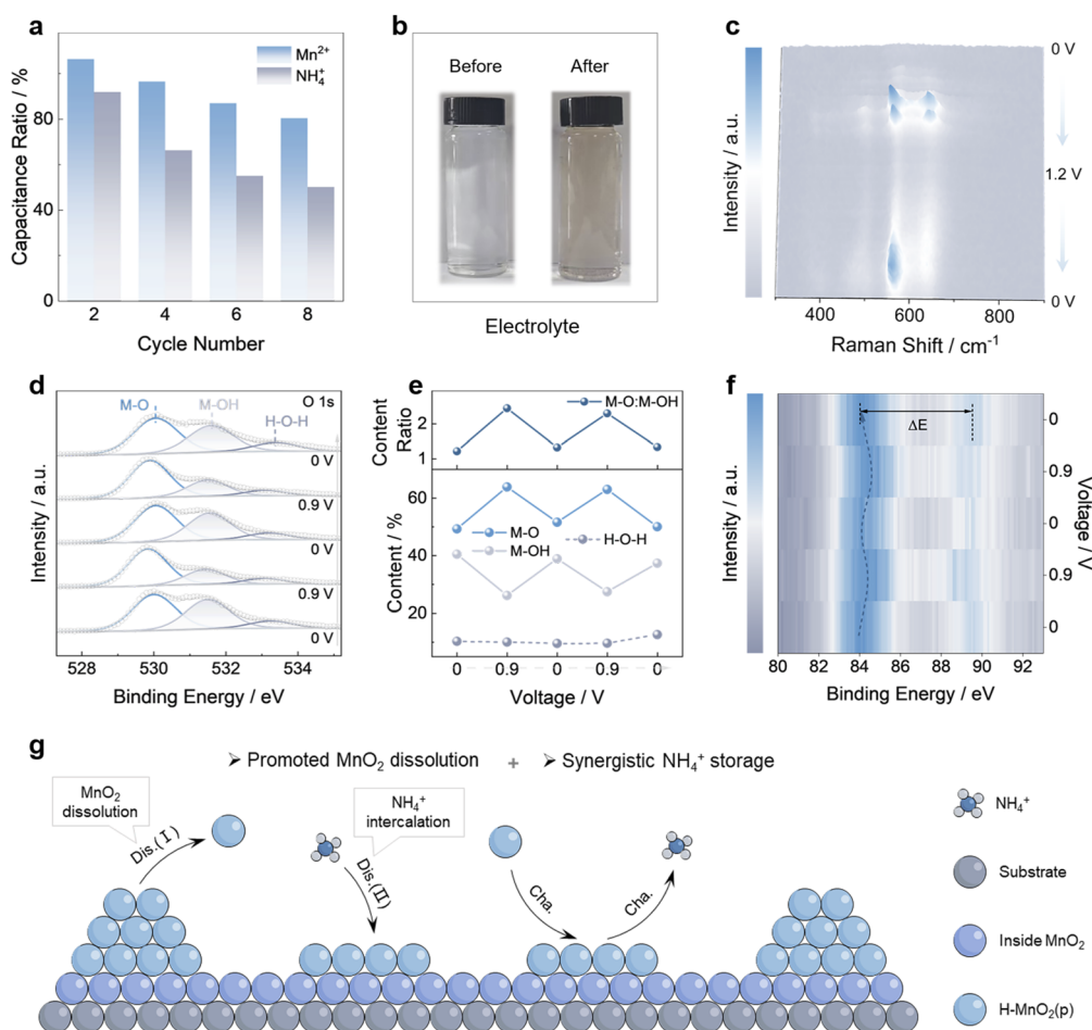
Fig. 4 Understanding the MnO 2 dissolution behavior assisted by \text{NH}_4^+ . (a) The capacitance ratio of the Rec-NM-MnO 2 electrode in the 0.5 M \text{Mn}(\text{NO}_3)_2 or 0.5 M (\text{NH}_4)_2\text{SO}_4 electrolyte to that in the \text{NH}_4^+ – \text{Mn}^{2+} mixed electrolyte at 2 mA cm -2 . (b) The digital images of (\text{NH}_4)_2\text{SO}_4 electrolyte before and after cycling. (c) Operando Raman contour map of Rec-NM-MnO 2 in 0.5 M (\text{NH}_4)_2\text{SO}_4 electrolyte. (d–f) Ex situ XPS characterization of the Rec-NM-MnO 2 electrode during the first two GCD cycles in the pure 0.5 M (\text{NH}_4)_2\text{SO}_4 electrolyte: (d) O 1s spectra; (e) content analysis of the O 1s spectra; (f) Mn 3s spectra. (g) Schematic diagram of the electrochemical behavior for Rec-NM-MnO 2 in the \text{NH}_4^+ – \text{Mn}^{2+} mixed electrolyte.
