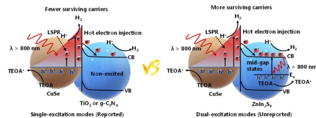
Fig. 4 Schematic of the newly developed plasmon-mediated photocatalysts using the earth-abundant copper chalcogenide (CuSe) for NIR-driven photocatalytic \text{H}_2 production. A possible band diagram and NIR-induced carrier dynamics in the plasmonic heterojunction are shown, illustrating the NIR light-driven photocatalytic reaction ( E_U : the energy of the band tail, also referred to as the Urbach energy).
