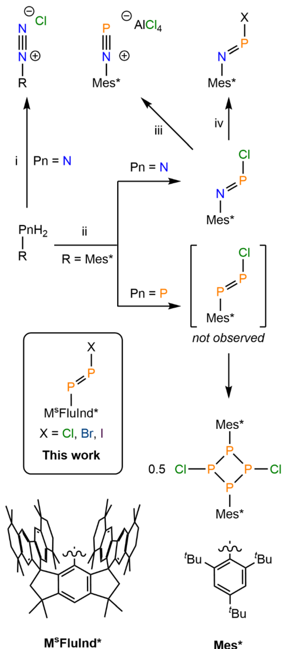
Fig. 1 General synthesis of [RNN][Cl] ( i = \text{excess HCl, excess NaNO}_2 ). Synthesis of (\text{Mes}^*)\text{NPCI} and [\text{ClP}(\mu\text{-PMes}^*)]_2 ( ii = \text{excess PCl}_3, \text{excess Et}_3\text{N} ). Synthesis of [(\text{Mes}^*)\text{NP}][\text{AlCl}_4] ( iii = \text{AlCl}_3 ). Synthesis of (\text{Mes}^*)\text{NPX} ( iv = \text{TMSX} ; \text{X} = \text{Br, I} ) reported herein. Structural diagrams of ligands \text{M}^s\text{FluInd}^* and \text{Mes}^* .
