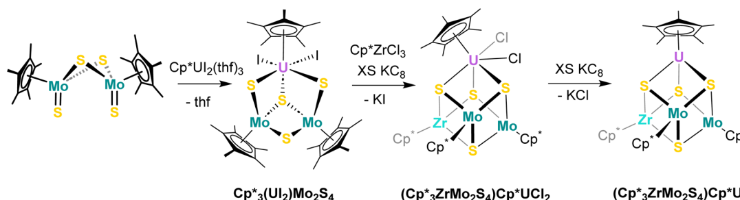
Scheme 2 Syntheses of \text{Cp}^*_3(\text{UI}_2)\text{Mo}_2\text{S}_4 , (\text{Cp}^*_3\text{ZrMo}_2\text{S}_4)\text{Cp}^*\text{UCl}_2 , and (\text{Cp}^*_3\text{ZrMo}_2\text{S}_4)\text{Cp}^*\text{U} .
