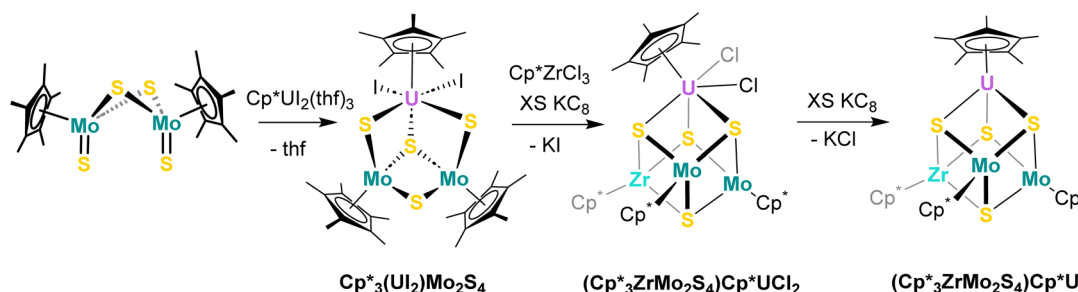
Scheme 2 Syntheses of \text{Cp}^*_3(\text{U}_2)\text{Mo}_2\text{S}_4 , (\text{Cp}^*_3\text{ZrMo}_2\text{S}_4)\text{Cp}^*\text{UCl}_2 , and (\text{Cp}^*_3\text{ZrMo}_2\text{S}_4)\text{Cp}^*\text{U} .
