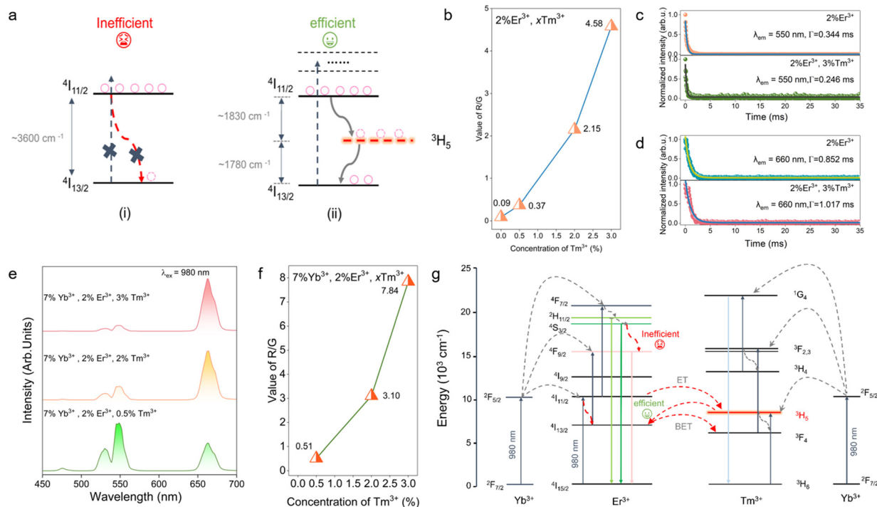
Fig. 2 (a) A schematic illustration of the regulatory role of the \text{Tm}^{3+}\text{-}^3\text{H}_5 energy level in UC emission of \text{Er}^{3+} . (b) R/G UC emission intensity ratio of GMTO: \text{Er}^{3+}, x\text{Tm}^{3+} ( x = 0\text{--}3\% ) under 980 nm excitation. (c) UC decay lifetimes of green emission at 550 nm of \text{Er}^{3+} in the GMTO: 2\%\text{Er}^{3+} and GMTO: 2\%\text{Er}^{3+}, 3\%\text{Tm}^{3+} under 980 nm excitation, respectively. (d) UC decay lifetimes of red emission at 660 nm of \text{Er}^{3+} in the GMTO: 2\%\text{Er}^{3+} and GMTO: 2\%\text{Er}^{3+}, 3\%\text{Tm}^{3+} under 980 nm excitation, respectively. (e) UC emission spectra of GMTO: 7\%\text{Yb}^{3+}, 2\%\text{Er}^{3+}, x\text{Tm}^{3+} ( x = 0.5\text{--}3\% ) under 980 nm excitation. (f) R/G UC emission intensity ratio of GMTO: \text{Yb}^{3+}, \text{Er}^{3+}, x\text{Tm}^{3+} ( x = 0.5\text{--}3\% ). (g) Schematic of UC emissions of GMTO: \text{Yb}^{3+}, \text{Er}^{3+}, \text{Tm}^{3+} upon 980 nm excitation.
