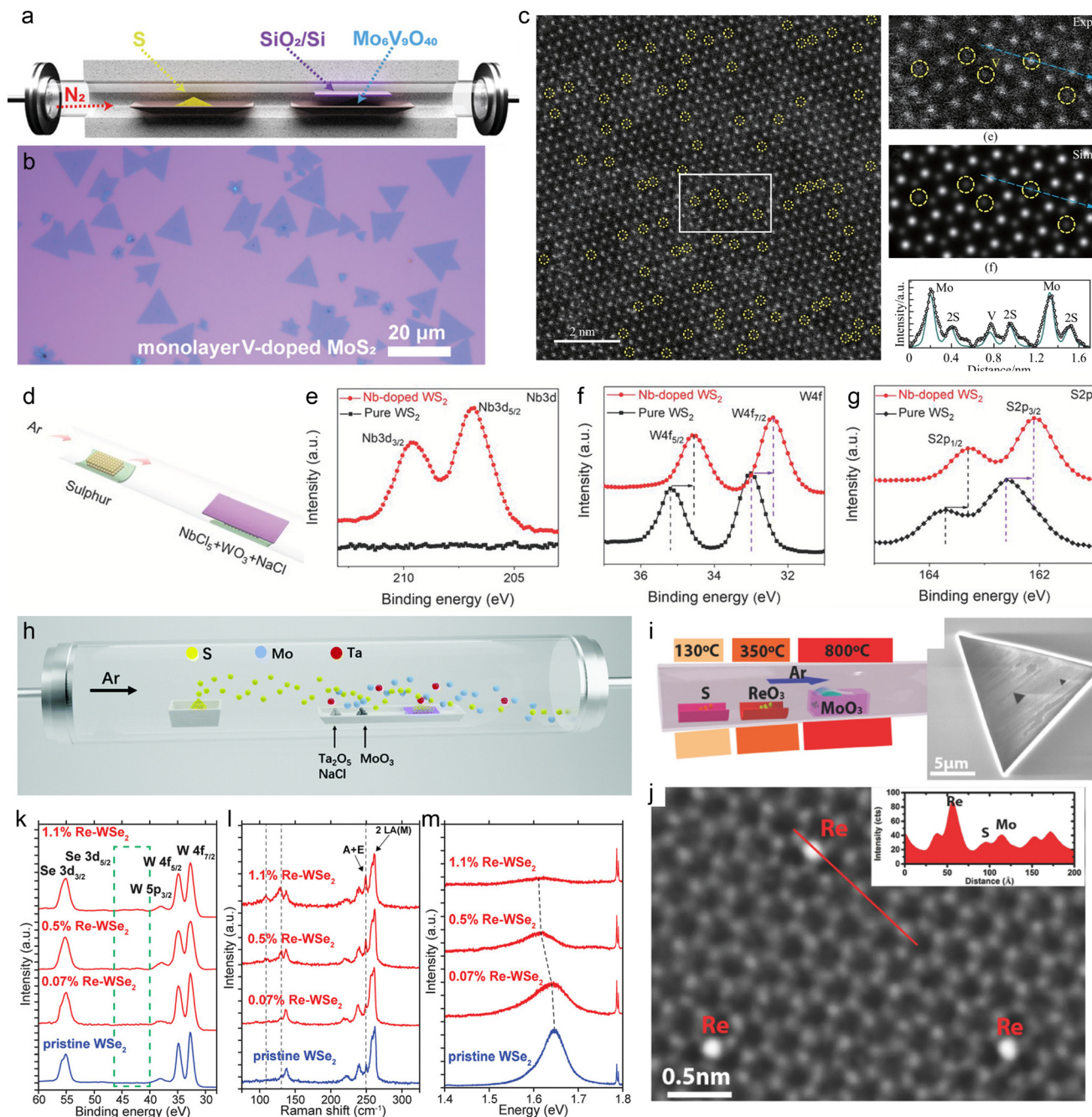
Fig. 6 Representative substitutional counter-doping across 2D TMDs. (a) Schematic image in CVD growth of V-doped \text{MoS}_2 using mixed oxide precursors ( \text{MoO}_3\text{--V}_2\text{O}_5 ) and S vapor and (b) OM image of the as-grown monolayer triangular flakes of V-doped \text{MoS}_2 with controlled V incorporation. (c) Atomic-resolution HAADF-STEM image of V-doped \text{MoS}_2 highlighting substitutional V atoms at Mo sites and the corresponding intensity line profile. (d) One-step Nb substitutional doping of \text{WS}_2 through \text{NbCl}_5 vapor transport and NaCl-assisted CVD, and (e–g) XPS spectra confirming Nb 3d, W 4f, and S 2p core-level shifts indicative of p-type behavior. (h) Schematic of Ta-doped \text{MoS}_2 synthesis using \text{Ta}_2\text{O}_5 and NaCl under an Ar flow, showing precursor distribution and one-zone CVD configuration. (i) Temperature-controlled in situ Re incorporation during \text{MoS}_2 CVD using \text{ReO}_3 and \text{MoO}_3 , displaying triangular monolayers and (j) atomic-resolution STEM image identifying Re atoms substituting Mo. (k–m) Substitutional Re-doping of \text{WSe}_2 via MOCVD, evidenced by XPS (W 4f, S 2p peaks), Raman red-shift, and PL quenching with increasing Re concentration. Reproduced from ref. 74 (panels a and b); ref. 76 (panel c); ref. 40 (panels d–g); ref. 26 (panel h); ref. 27 (panel i and j); and ref. 88 (panels k–m) under Creative Commons license (CC BY).
