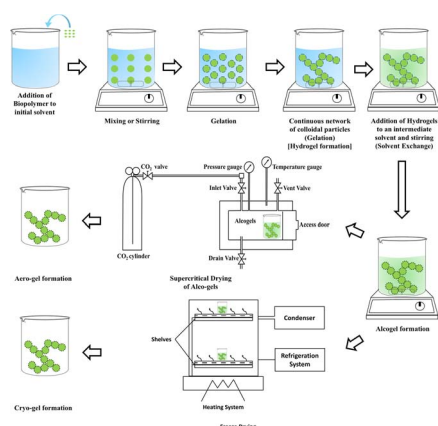
Fig. 2 Steps for the formation of aerogel using solvent exchange method.
