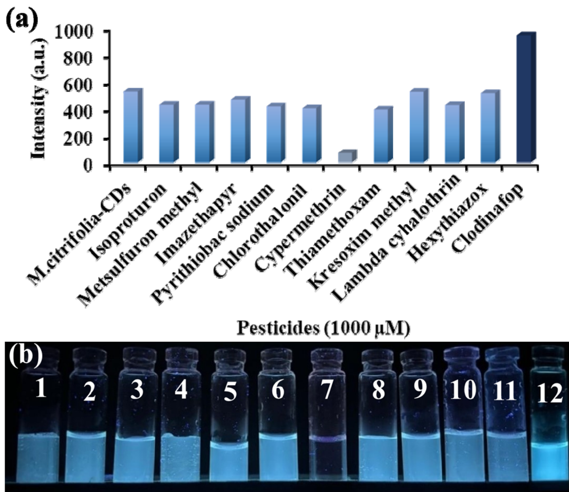
Fig. 4 (a) Fluorescence emission spectra of M. citrifolia -CDs at an emission wavelength of 456 nm with the addition of various pesticide (isoproturon, metsulfuron methyl, imazethapyr, pyriethion sodium, chlorothalonil, cypermethrin, thiamethoxam, kresoxim methyl, lambda cyhalothrin, hexythiazox, and clodinafop) solutions. (b) Variation in the fluorescence intensities of M. citrifolia -CD solutions in the presence of different pesticides under a UV lamp at 365 nm (1 – M. citrifolia -CDs, 2 – isoproturon, 3 – metsulfuron methyl, 4 – imazethapyr, 5 – pyriethion sodium, 6 – chlorothalonil, 7 – cypermethrin, 8 – thiamethoxam, 9 – kresoxim methyl, 10 – lambda cyhalothrin, 11 – hexythiazox, and 12 – clodinafop).
