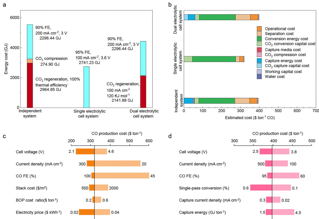
Fig. 75 (a) Comparative schematic of energy consumption for the production of 100 tons of CO across various systems. (b) Techno-economic assessment (TEA)-based estimation of CO production costs. (c) and (d). Sensitivity analysis of CO production costs for a single electrolytic cell system and a dual electrolytic cell system, respectively, based on optimistic and pessimistic parameter assumptions. Reprinted (adapted) with permission from ACS Energy Lett. 2023, 8(6), 2840–2857. Copyright © 2023 American Chemical Society.
