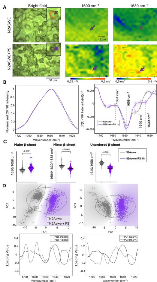
Fig. 5 PS-induced changes in \beta -sheet structures in an AD cellular model. (A) Bright-field image and hyperspectral O-PTIR maps of N2A5we cells exposed or unexposed to PS, acquired at 1600 cm -1 (PS-specific signal), 1630 cm -1 ( \beta -sheet content), normalized to 1658 cm -1 (total protein/ \alpha -helices). PS-exposed cells showed increased intensity at 1630 cm -1 (purple arrow) compared to non-exposed control (grey arrow). Inset: Magnified view of the demarcated cellular region used for spectral analysis. (B and C) Quantification of secondary structure components from second-derivative spectra of the amide I region. Ratios were calculated between 1630 cm -1 and 1658 cm -1 (total \beta -sheets) and 1694 cm -1 and 1658/1630 cm -1 (antiparallel \beta -sheets). (D) Principal component analysis (PCA) of amide I spectra (1610–1710 cm -1 ) showing clear separation between PS-exposed and control N2A5we cells. PCA loading plots indicated that wavenumbers corresponding to \beta -sheet structures contributed most strongly to group differentiation (data derived from n = 5 (control) and n = 6 (PS-exposed) individual cells, totaling >4000 spectra). Statistical significance determined by Mann–Whitney U test.
