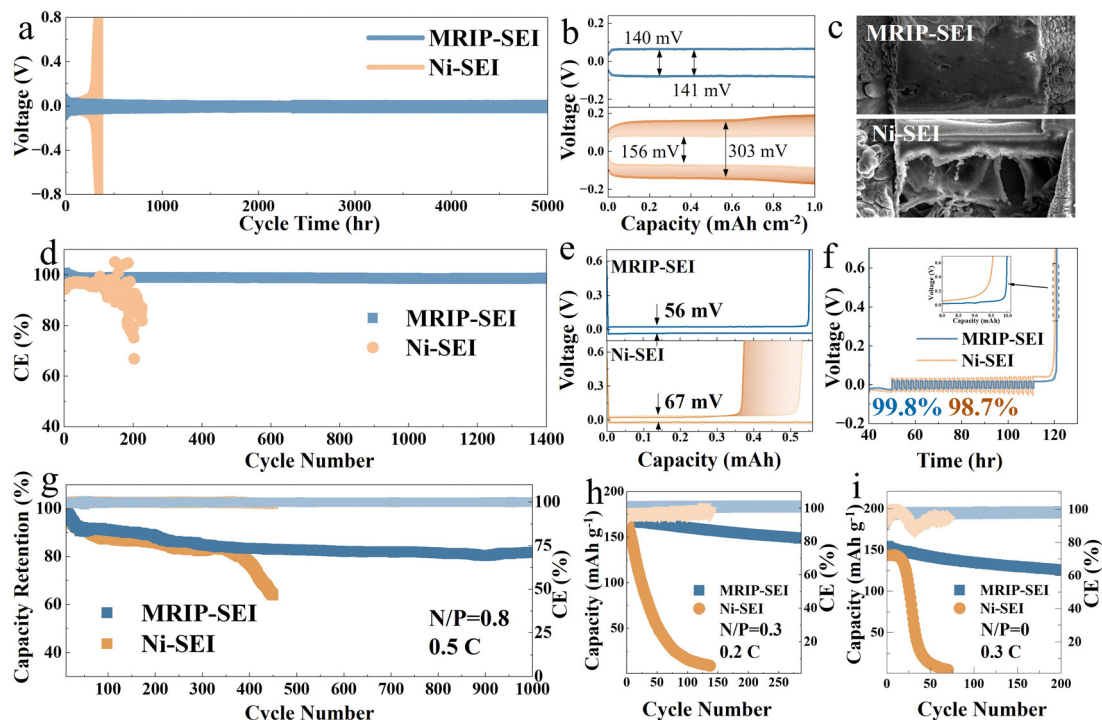
Fig. 6 MRIP-SEI to optimize interfacial mass transfer for high-performance anode-free and anode-less lithium batteries. (a) Comparison of cycling performance and (b) charging/discharging curves of Li||Li symmetrical cells at 2 \text{ mA cm}^{-2} . (c) FIB-SEM images with the MRIP-SEI and Ni-SEI after cycling. (d) Comparison of cycle performance of Li||Cu cells and (e) corresponding charging/discharging curves at 0.5 \text{ mA cm}^{-2} . (f) Aurbach average CE of Li||Cu cells at 2 \text{ mA cm}^{-2} . (g) Cycling performance of Cu@Li||LFP full cells at 0.5C ( N/P \sim 0.8 ). (h) Cycling performance of anode-less Cu@Li||LFP full cells at 0.2C ( N/P \sim 0.3 ). (i) Cycling performance of anode-free Cu||LFP full cells at 0.3C ( N/P = 0 ).
