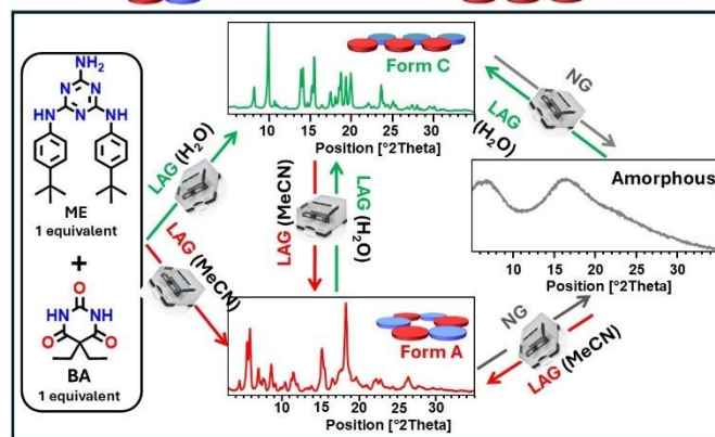
Figure 38 Polymorph interconversion of 1:1 ME:BA cocrystals by ball milling. NG milling of 1:1 ME:BA consistently yields the amorphous form. LAG with MeCN produces Form A (rosette), whereas LAG with water produces Form C (linear tape). All three forms can be obtained directly by milling an equimolar mixture of ME and BA to steady-state. 67 Adapted from ref. 67 with permission from The Royal Society of Chemistry.
