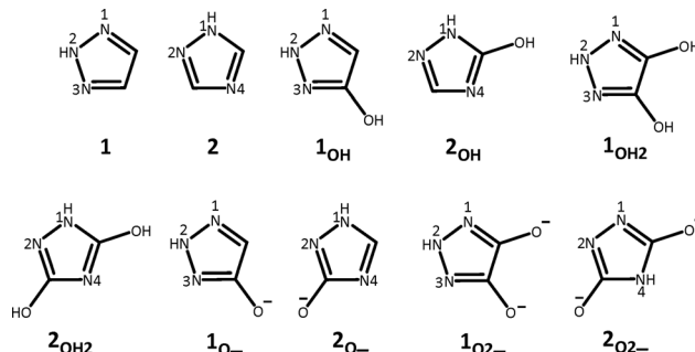
Fig. 1 Neutral, anionic, and dianionic systems considered for CO 2 capture.
