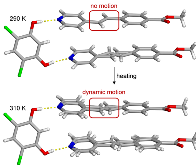
Fig. 1 X-ray crystal structures of ( 4,6-diCl-Res )-2( PEB ) illustrating the disorder upon heating within PEB . The O-H...N hydrogen bonds are shown with yellow dashed lines. The 290 K data is from the original report, 12 while the 310 K data is from this work. The red rectangle highlights a change in disorder and motion.
