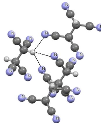
Fig. 3 Fragment of the crystal structure of 1,1,2,2-ethantetracarbonitrile (BUGKIX01 ref code). 82 The H...N intermolecular contacts are designated by the black narrow lines.
