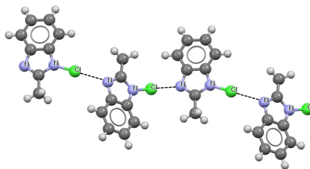
Fig. 4 Fragment of the crystal structure of 1-chloro-2-methyl-1 H -benzimidazole (GEKPIZ ref code). 84 The Cl \cdots N intermolecular contacts are designated by the black narrow lines.
