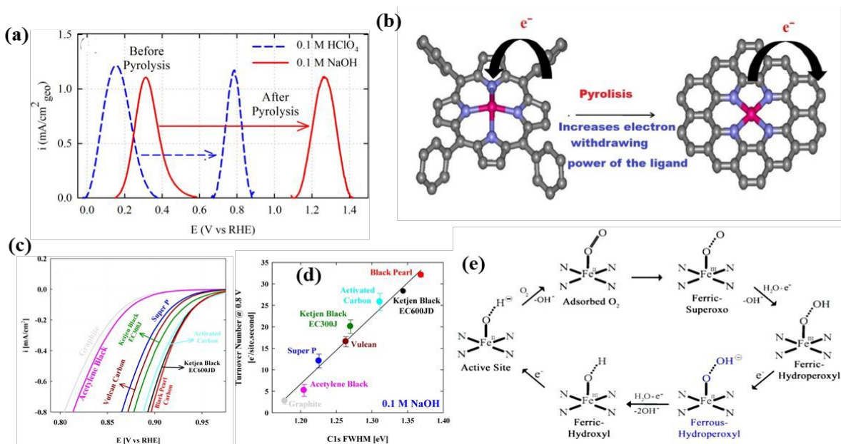
Fig. 3. (a) Square-wave voltammetry profiles of Fe-N_4 catalyst supported on black pearl carbon before and after pyrolysis at 800 °C in 0.1 M HClO_4 and 0.1 M NaOH electrolytes. (b) Structural models of active site structures before and after pyrolysis at 800 °C. Color codes in structural models: red, iron; blue, nitrogen; gray, carbon; white, oxygen. (c) ORR activity of Fe-N_4 catalyst (pyrolyzed at 800 °C) on various carbon supports in O_2 -saturated 0.1 M NaOH electrolyte at 900 rpm rotation rate and 20 mV s -1 scan rate. (d) Linear relationship between ORR turnover numbers in 0.1 M NaOH electrolyte versus full-width at half-maximum of C 1s photoemission spectra. (e) Catalyst cycle showing the redox mechanism involved in ORR on pyrolyzed Fe-N_4/C active sites in dilute alkaline medium. Reproduced from ref. 79 with permission from the American Chemical Society, copyright 2013.
