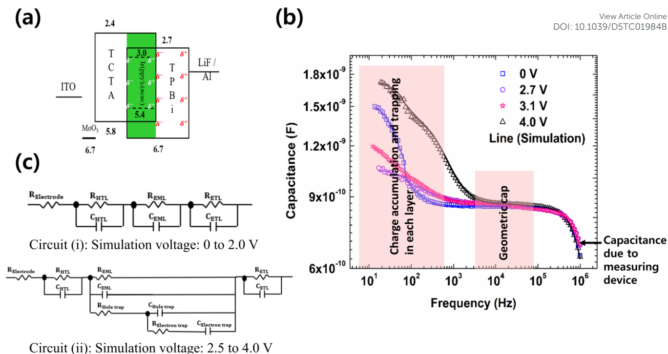
Fig. 8 (a) The schematic energy-level diagram of the mixed-host EML OLED device. (b) The capacitance-frequency measurement curves at different voltages. (c) Modeled equivalent circuits for different voltage simulations. Reproduced with permission from Ref. 37 Copyright 2023, Elsevier Ltd.
