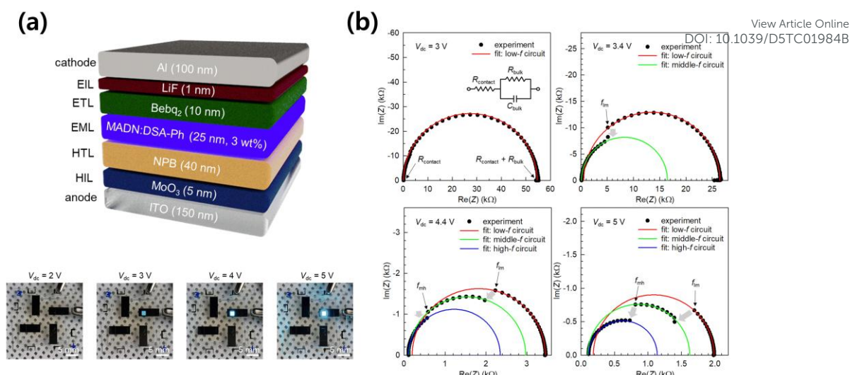
Fig. 14 (a) The schematic illustration of the OLED structure and the photographs showing the gradual switching and brightness emission of the fabricated OLED. (b) Cole-Cole plot of the OLED measured at 3 to 5 V. Reproduced with permission from Ref. 83 Copyright 2023, Royal Society of Chemistry.
