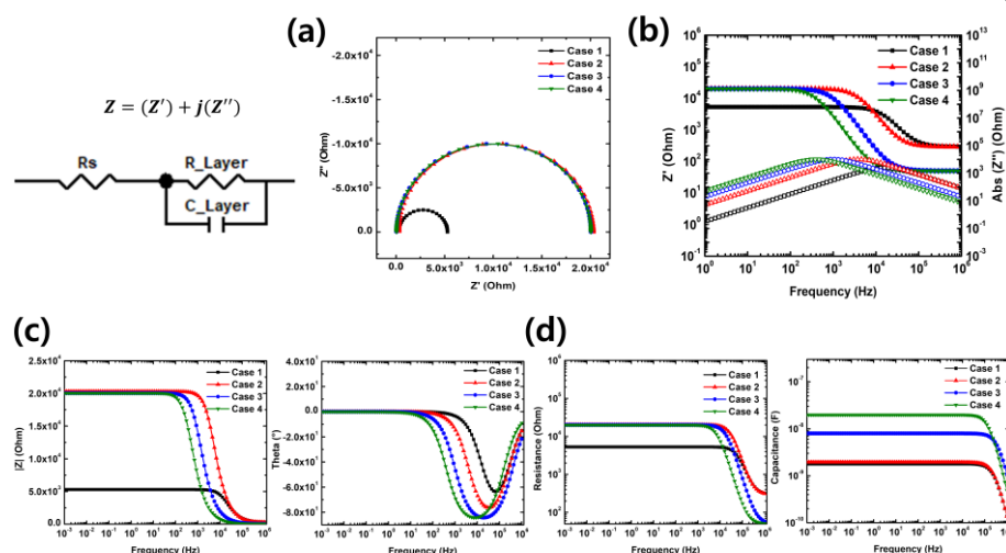
Fig. 4 The simulation results from Zview software using the one RC unit circuit and the values from (Table 1) are presented in different impedance spectra. (a) Nyquist (Cole-Cole) plot. (b) Impedance-frequency ( Z - F ) dependent plot. (c) Absolute impedance-frequency ( |Z - F ) and phase ( \phi )-frequency-dependent plots. (d) The Bode plot constituting: Resistance-frequency ( R - F ) and capacitance-frequency ( C - F ) plots.
