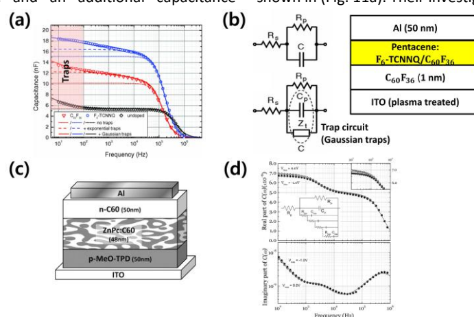
Fig. 11 (a) Capacitance spectra of pentacene Schottky diodes, comprising 0.5 wt.% each of C_{60}F_{36} and F_6 -TCNNQ dopant molecules and undoped device at 0 V. Reproduced with permission from Ref. 79 Copyright 2013, American Physical Society. (b) The applied equivalent circuit models, with and without the trap distribution element ( Z_t ) for simulating the capacitance-frequency dependent spectra and the device structure. Reproduced with permission from Ref. 79 Copyright 2013, American Physical Society. (c) Structure of the solar cell device (ZnPc:C60 bulk heterojunction as photo-active layer) Reproduced with permission from Ref. 80 Copyright 2012, AIP Publishing. (d) The real and imaginary parts of the complex capacitance at 0 V and -1.0 V bias. Reproduced with permission from Ref. 80 Copyright 2012, AIP Publishing.
