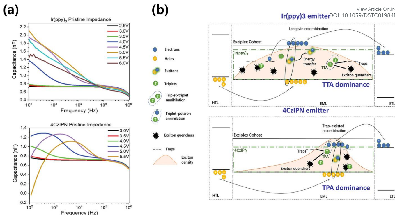
Fig. 17 (a) Capacitance-frequency plot of the \text{Ir(ppy)}_3 - and 4CzIPN-based devices. (b) TTA and TPA degradation and quenching mechanisms in a phosphorescent emitter ( \text{Ir(ppy)}_3 ) and thermally activated delayed fluorescent emitter (4CzIPN), respectively. Reproduced with permission from Ref. 58 Copyright 2024, Wiley-VCH.
