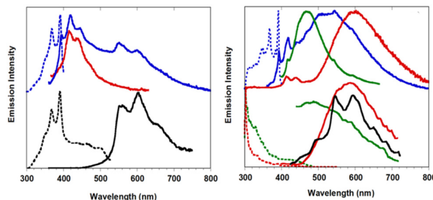
Fig. 11 Powders of 3Br left: at 298 K. Top: Prompt emission ( \lambda_{\text{exc}} = 280 nm, red solid line; \lambda_{\text{exc}} = 340 nm, blue solid line) and excitation profiles ( \lambda_{\text{em}} = 420 nm, dashed blue line). Bottom: Delayed emission ( \lambda_{\text{exc}} = 340 nm, 1 ms delay, window 50 ms; black solid line) and excitation profiles ( \lambda_{\text{em}} = 550 nm, dotted black line). Right: at 77 K. Top: prompt emission ( \lambda_{\text{exc}} = 280 nm, red solid line; \lambda_{\text{exc}} = 340 nm, blue solid line; \lambda_{\text{exc}} = 385 nm, green solid line) and excitation profiles ( \lambda_{\text{em}} = 420 nm, dotted blue line). Bottom: delayed emission ( \lambda_{\text{exc}} = 360 nm, 100 \mu\text{s} delay, window 500 \mu\text{s} , red solid line; \lambda_{\text{exc}} = 385 nm, 100 \mu\text{s} delay, window 500 \mu\text{s} , green solid line; \lambda_{\text{exc}} = 385 nm, 5 ms delay, window 10 ms, black solid line) and excitation profiles ( \lambda_{\text{em}} = 523 nm, dotted green line; \lambda_{\text{em}} = 600 nm, dotted red line). Adapted with permission from ref. 69. Copyright 2018, John Wiley and Sons.
