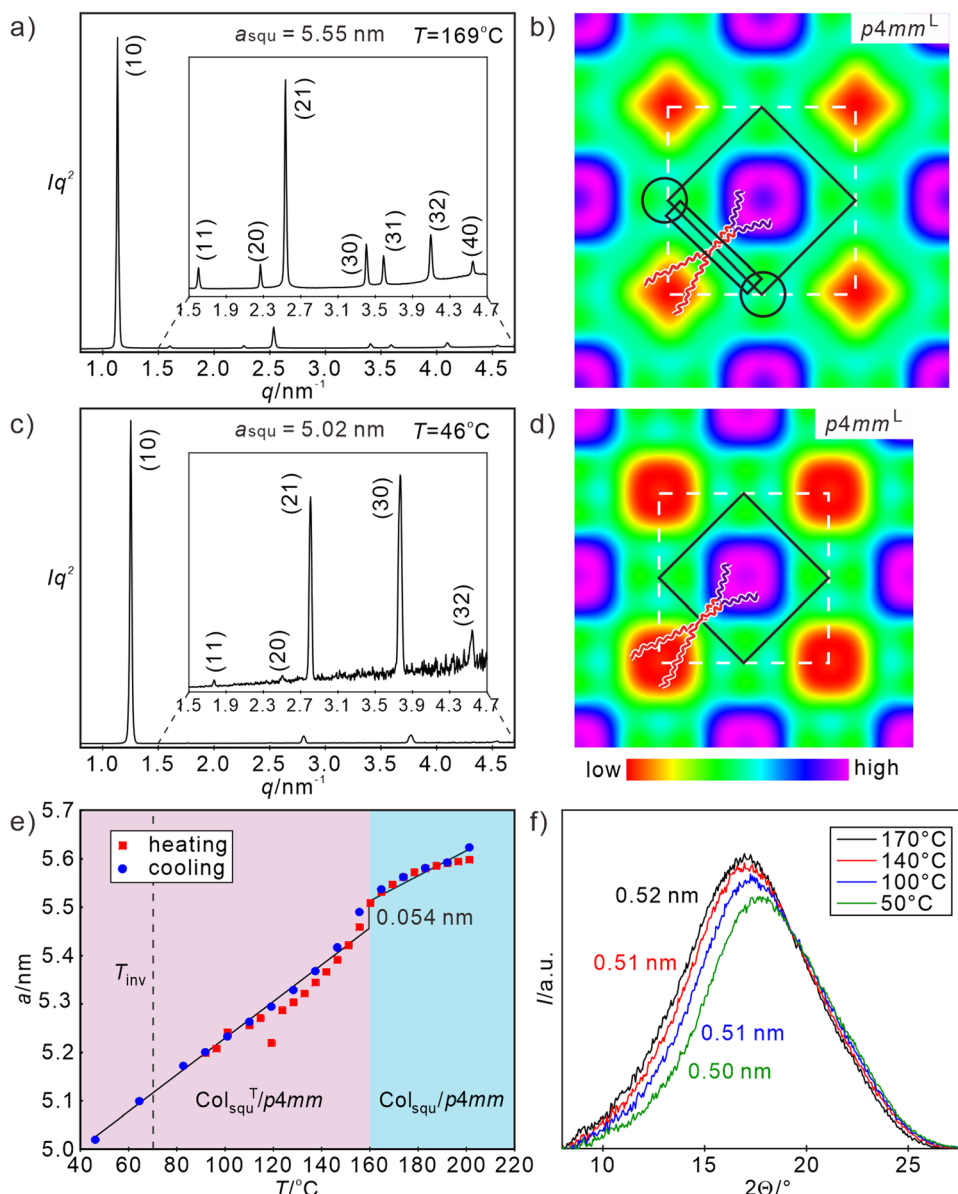
Fig. 3 (a) and (c) SAXS patterns (for numerical data, see Tables S8 and S9, ESI†) and (b) and (d) reconstructed ED maps of the \text{Col}_{\text{squ}}/\text{p4mm}^{\text{L}} phase of H8/16 at 169 ^\circ\text{C} and 46 ^\circ\text{C} , respectively (phase choices 00\pi 0\pi\pi\pi and 00\pi 0\pi\pi ); white dashed lines indicate the unit cell and solid black lines the shape of one honeycomb cell, in (b) a molecular model is drawn, black rectangle indicates the aromatic core and the black circles indicate the glycerol nodes; (e) shows the temperature dependence of a_{\text{squ}} ; (f) shows the diffuse WAXS scatterings at different temperatures (for numerical WAXS data, see Table S1, ESI†). For DSC data and textures, see Fig. S1d and S4 (ESI†).
