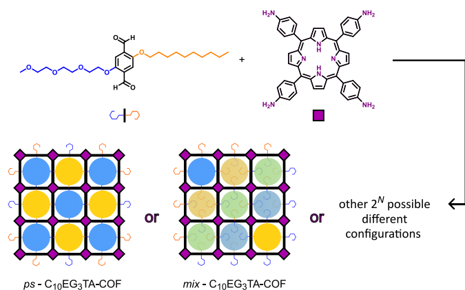
Figure 1: Schematic representation of the COF synthesis from a C 10 EG 3 TA functionalized linker and 5,10,15,20-tetrakis(4-aminophenyl)-21H,23H-porphyrin, showing the formation of ps -C 10 EG 3 TA-COF, mix -C 10 EG 3 TA-COF, and other possible configurations depending on the linker arrangement.
