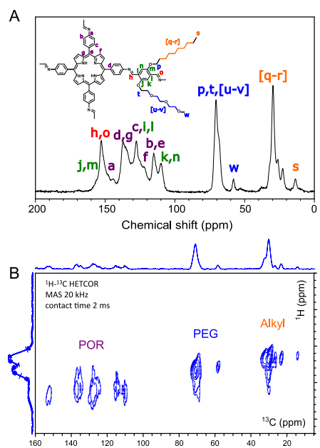
Figure 4: A) Solid-state ^{13}\text{C} CP/MAS NMR spectrum of the COF with carbon signal assignments. B) ^1\text{H} - ^{13}\text{C} HETCOR spectra showing C-H correlations for the EG, alkyl, and porphyrin units.
