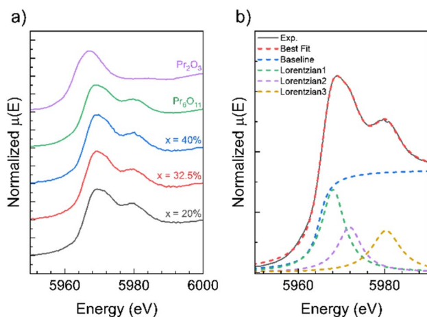
Fig. 6 (a) Pr L_{3/2} absorption of Pr in \text{Ce}_x(\text{SmPrLaY})_{1-x}\text{O}_{2-\delta} and measured standards and (b) an example of fitting procedure performed on \text{Pr}_6\text{O}_{11} .
