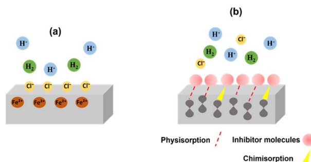
Fig. 13 Illustration of the corrosion process of MS in 1 M HCl (a) in the absence of the inhibitor (b) in the presence of the combined AC–QR extract as a green corrosion inhibitor.
